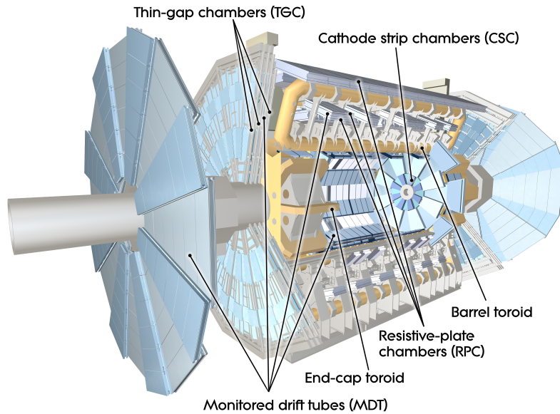
Figure 3.8: Schematic layout of the ATLAS muon spectrometer consisting of high precision MDT and CSC chambers as well as RPC and TGC trigger chambers [84].
