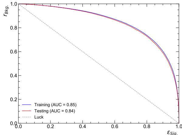
Figure 8.8: Receiver operating characteristic of the ML classifier. The events are separated into training and test set. Both curves are in good agreement, which indicates that the NN is not overtrained. The quantity in the legend denotes the area under the curve (AUC) and is a metric for the overall performance of the classification problem.
