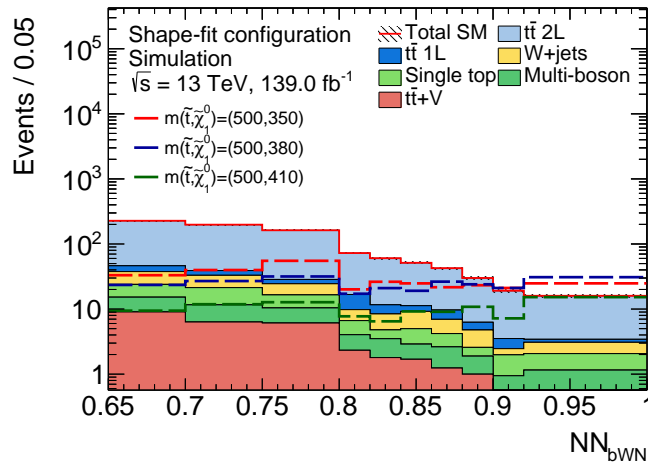
Figure 8.18: Distribution of \text{NN}_{\text{bWN}} in the range from 0.65 to 1.0 for SM background as well as for signal points with three different mass splittings. An additional requirement on m_T > 150 GeV is applied on the first three bins ranging from 0.65 to 0.8. Only the statistical uncertainty of the simulated events is shown in the shaded area around the total SM expectation. The t\bar{t} background is not yet normalised to the CR.
