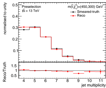
(a) Jet multiplicity
