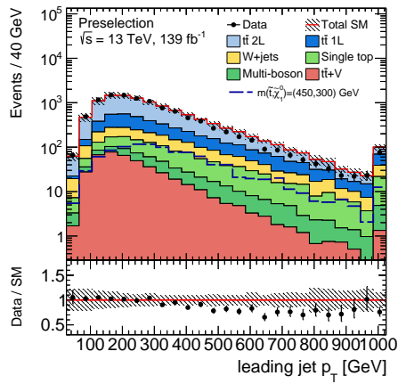
(c) Leading jet p_T
