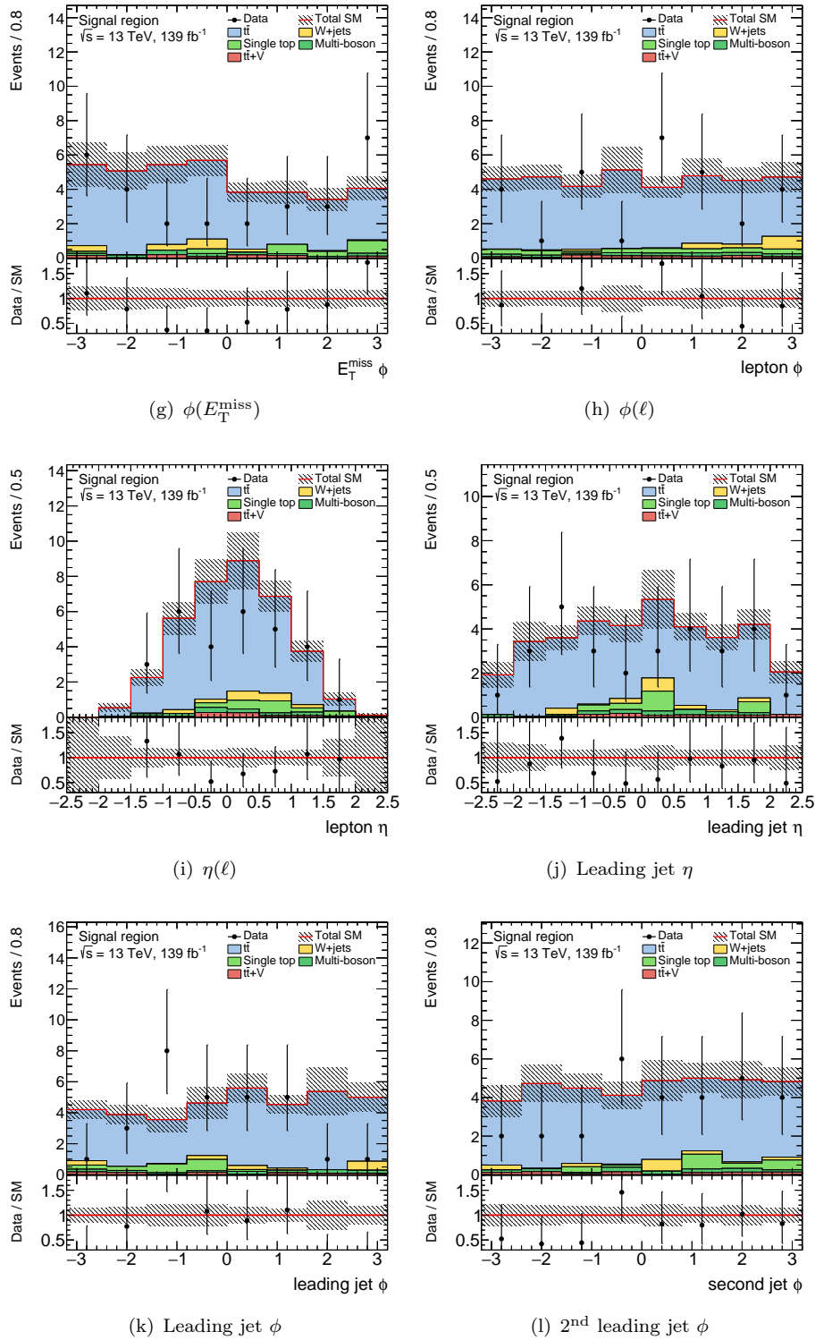
Figure A.5: Kinematic distributions of selected observables in the signal region. The t\bar{t} background processes are scaled by the normalisation factor obtained from a likelihood fit of the CR, while all other SM background processes are normalised with the respective theoretical cross section. The shaded band around the total SM prediction as well as the shaded band in the data/SM ratio include statistical and systematic uncertainties. Overflows are included in the last bin.
