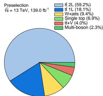
Figure 8.1: Relative contributions of the individual SM backgrounds after the preselection.
