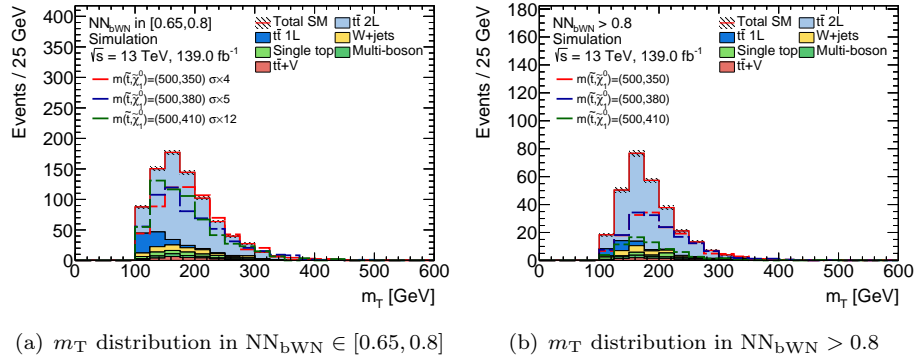
(a) m_T distribution in \text{NN}_{\text{bWN}} \in [0.65, 0.8]
