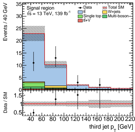
(e) 3 rd leading jet p_T
