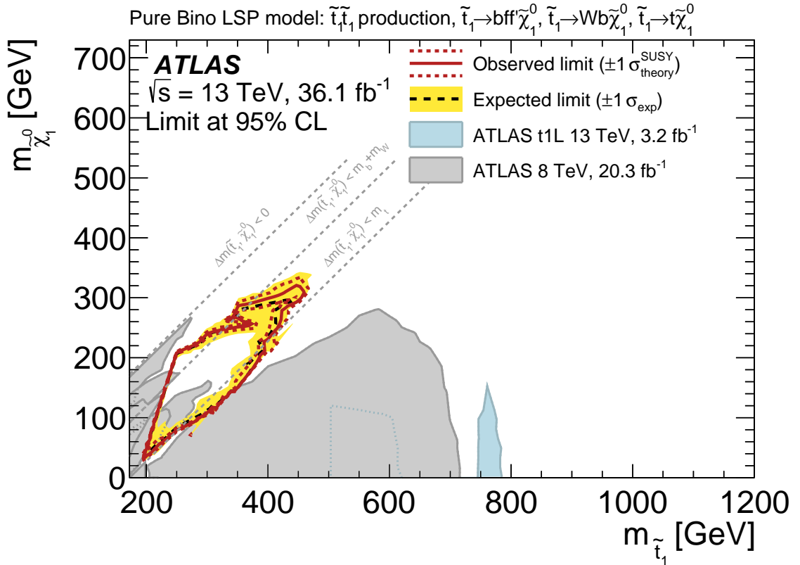
Figure 7.13: Expected (black dashed) and observed (red solid) exclusion limit at 95 % confidence level in the phase space spanned by m(\tilde{\chi}_1^0) versus m(\tilde{t}_1) for direct top squark pair production. Either \tilde{t}_1 \rightarrow t\tilde{\chi}_1^0 , \tilde{t}_1 \rightarrow bW\tilde{\chi}_1^0 , or \tilde{t}_1 \rightarrow bff'\tilde{\chi}_1^0 decay modes with a branching ratio of 100 % are assumed. The excluded regions from previous publications [55, 173] are illustrated with the grey and blue shaded area, respectively.
