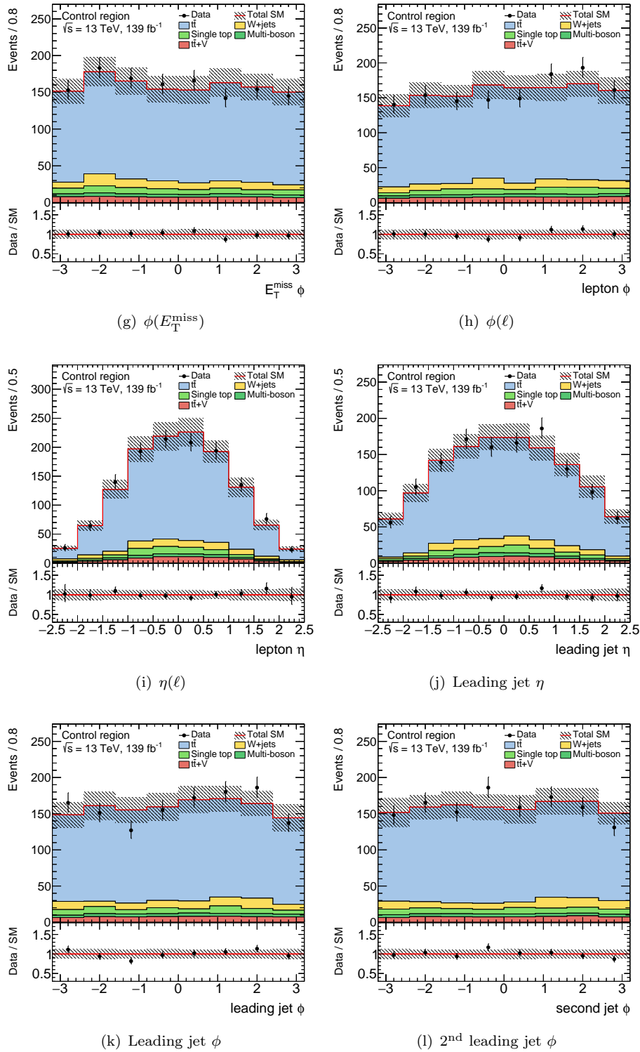
Figure A.3: Kinematic distributions of selected observables in the control region. The t\bar{t} background prediction is scaled by the normalisation factor obtained from a likelihood fit of the CR, while all other SM background processes are normalised with the respective theoretical cross section. The hatched band around the total SM prediction and the hatched band in the data/SM ratio include statistical and systematic uncertainties, except for the t\bar{t} modelling uncertainties, which are only defined for the signal and validation region. Overflows are included in the last bin.
