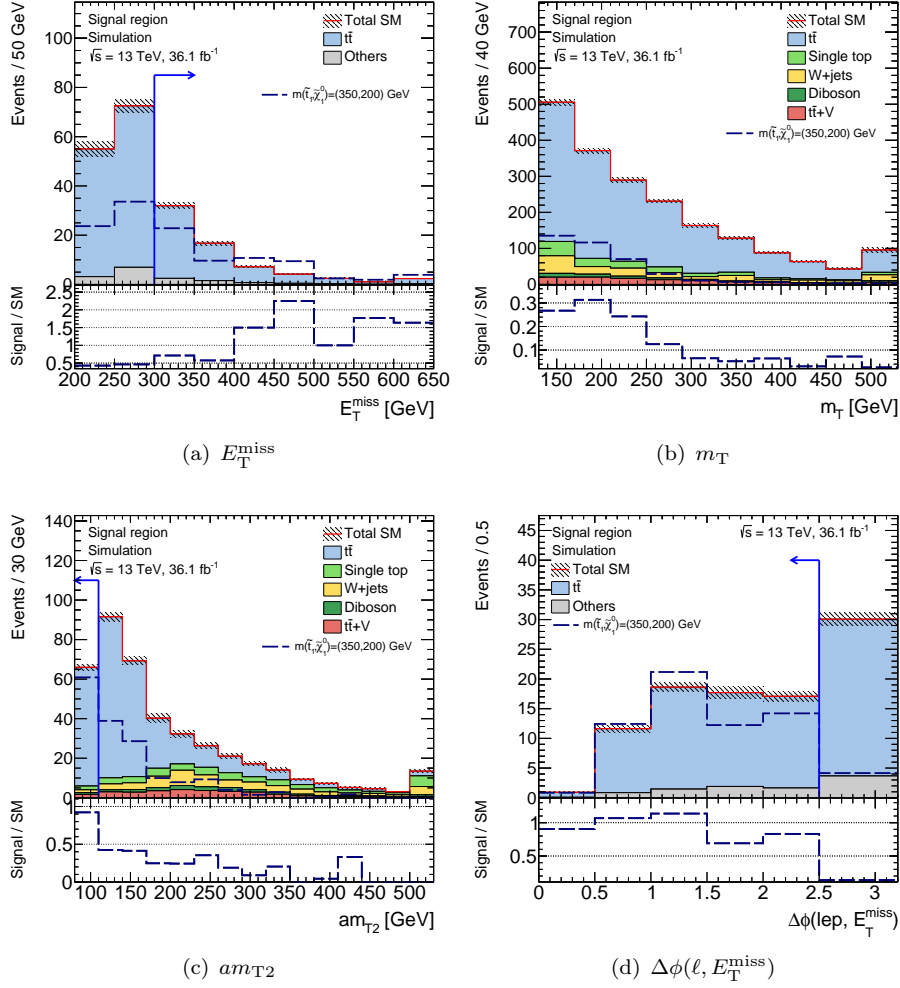
Figure 7.5: Kinematic distributions of the variables used to define the signal region. The selection on the displayed quantity is omitted as indicated by the vertical line, except for the distribution of the m_T variable, because a tight requirement on m_T is already applied at event preselection level. The direction of the arrow on top of the vertical line indicates the region of accepted events in the signal region. Only statistical uncertainties are included. The category 'Others' in the legend represents the sum of minor SM backgrounds that contribute less than 5 % of the total SM background. The lower panel shows the ratio of signal to SM background in each bin respectively.
