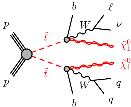
Figure 2.4: Simplified model topology of direct top squark pair production in a kinematically compressed phase space, referred to as 3-body decay scenario. The decay structure is characterised by m(W) + m(b) < \Delta m < m(t) . The top quark is produced off-shell and thus the top squarks directly decay to a b quark, W boson and the neutralino LSP. By courtesy of the ATLAS supersymmetry physics analysis group.
