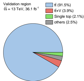
Figure 7.8: Relative contributions of the individual SM backgrounds in the validation region.
