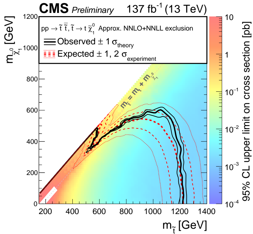
Figure 9.3: Expected (red dashed) and observed (black solid) 95% exclusion limit for top squark pair production [203] in the plane spanned by m(\tilde{t}_1) and m(\tilde{\chi}_1^0) . Thin red dashed lines indicate the \pm 1, 2 \sigma_{\text{experiment}} uncertainty in the expected limit. The thin black lines represent the \pm 1 \sigma_{\text{theory}} uncertainty based on the theoretical uncertainties on the signal cross section.
