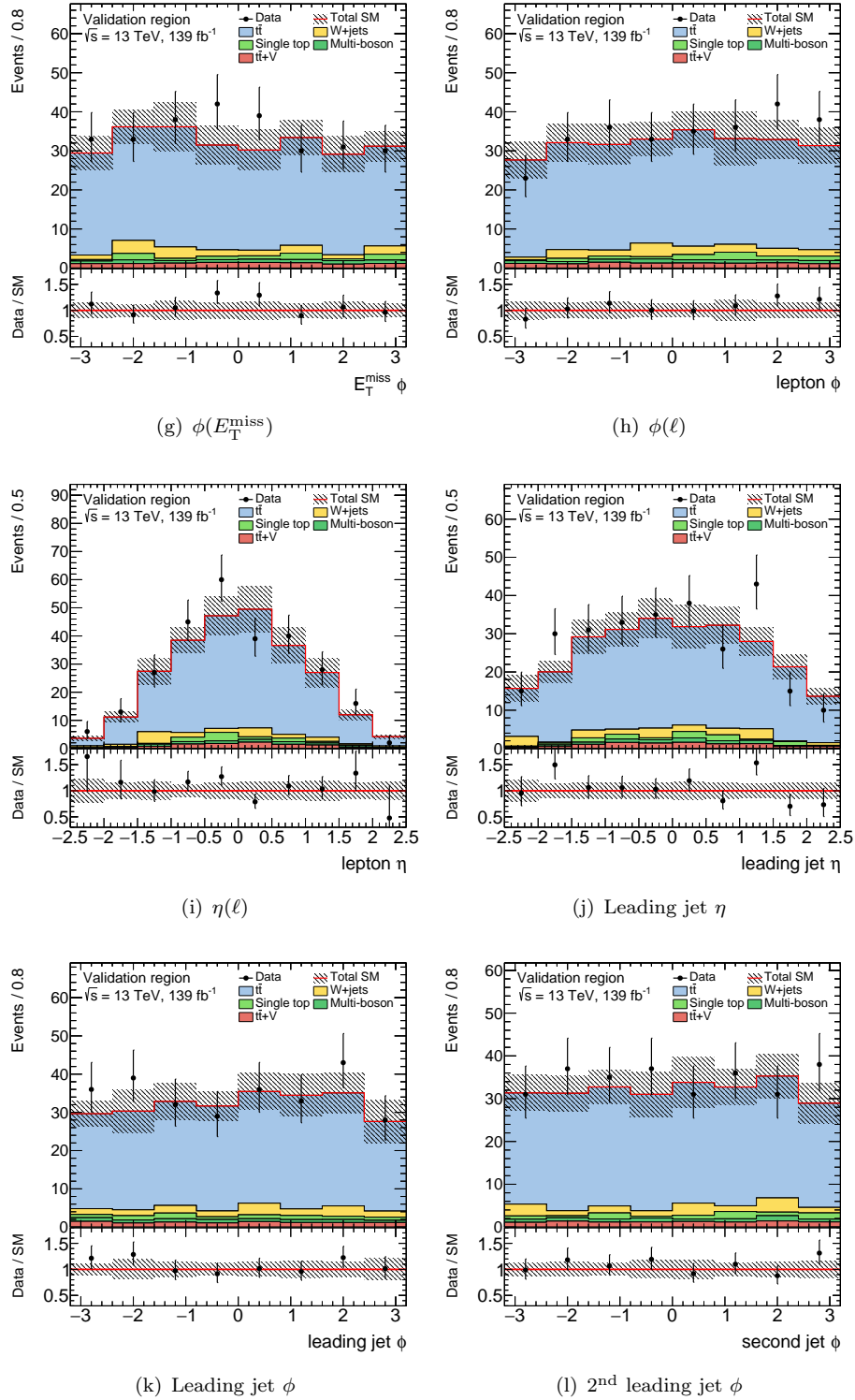
Figure A.4: Kinematic distributions of selected observables in the validation region. The t\bar{t} background processes are scaled by the normalisation factor obtained from a likelihood fit of the CR, while all other SM background processes are normalised with the respective theoretical cross section. The shaded band around the total SM prediction as well as the shaded band in the data/SM ratio include statistical and systematic uncertainties. Overflows are included in the last bin.
