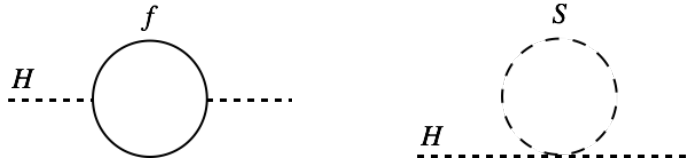
Figure 2.1: One-loop corrections to M_h^2 . For a fermion f (left) and a scalar particle S (right) [28].
