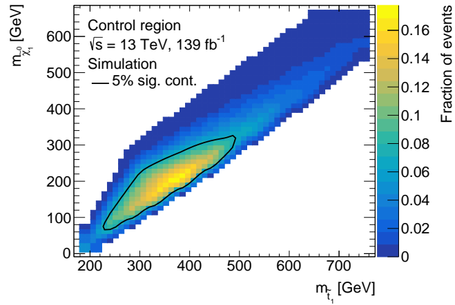
Figure 8.20: Signal contamination in the control region illustrated in the phase space spanned by m(\tilde{t}_1) versus m(\tilde{\chi}_1^0) . The black contour line illustrates the threshold for a signal fraction of 5%. Signal points where the contamination is above 5% are already excluded by previous analyses.
