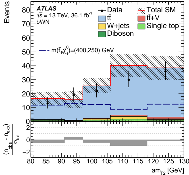
Figure 7.12: Kinematic distribution of am_{T2} for the shape-fit scenario. The event selections corresponding to the bins of the shape-fit are applied. t\bar{t} events are scaled with the normalisation factor obtained from the control region. Statistical and systematic uncertainties are included. The last bin contains overflows. Additionally, the benchmark signal model is overlaid for comparison. The bottom panel shows the difference between observed and predicted events divided by the total uncertainty ( \sigma_{\text{tot}} ).
