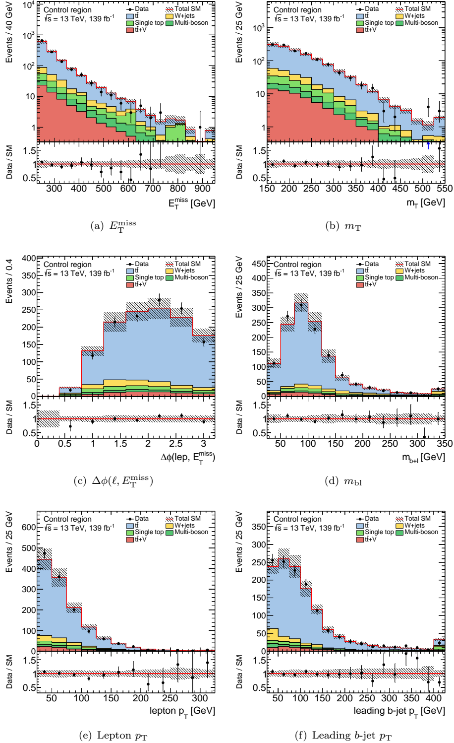
Figure 8.21: Kinematic distributions of selected observables in the control region. The t\bar{t} background prediction is scaled by the normalisation factor obtained from a likelihood fit of the CR, while all other SM background processes are normalised with the respective theoretical cross section. The hatched band around the total SM prediction and the hatched band in the data/SM ratio include statistical and systematic uncertainties, except for the t\bar{t} modelling uncertainties, which are only defined for the signal and validation region. Overflows are included in the last bin.
