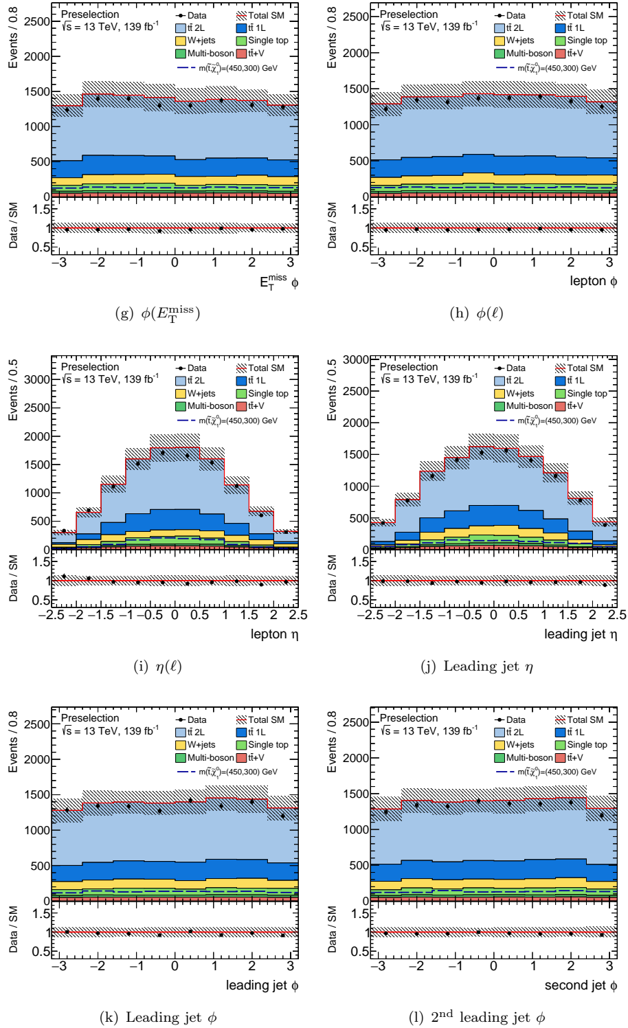
Figure A.1: Kinematic distributions of key observables after the preselection is applied. The t\bar{t} background prediction is scaled by the normalisation factor obtained from a likelihood fit of the CR, while residual SM background processes are normalised with the respective theoretical cross-section. The hatched area around the total SM prediction and the hatched band in the ratio include statistical and systematic uncertainties, except for the t\bar{t} modelling uncertainties, which are defined only for the signal and validation region. Additionally, the expected distribution of the SUSY benchmark signal model is overlaid (blue dashed line). Overflows are included in the last bin.
