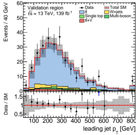
(c) Leading jet p_T
