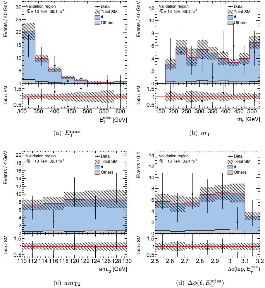
Figure 7.9: Kinematic distributions of key variables in the validation region. The t\bar{t} events are scaled by the normalisation factor obtained in the CR. Residual SM background processes are normalised with the respective theoretical cross section. The category ‘Others’ in the legend represents the sum of minor SM backgrounds that contribute less than 5 % of the total SM background. The lower panel shows the ratio of data to the SM prediction. The uncertainty band includes statistical and systematic uncertainties. The last bins include the overflow.
