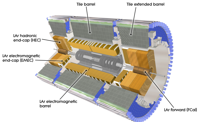
Figure 3.7: Assembly of the electromagnetic and hadronic calorimeter system in the ATLAS experiment [83].
