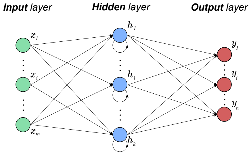
Figure 5.3: Basic concept of a recurrent neural network. In addition to standard connections between various layers, cyclic connections in hidden layers are allowed. As a consequence, a RNN is able to process not only the information from the current input neuron, but also from previous inputs. This means that sequential data as well as inputs of variable length can be handled. For simplicity the bias neurons are omitted.
