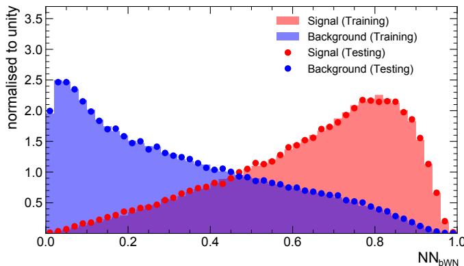
Figure 8.7: Distribution of the ML output score, referred to as NN_{bWN} . The events are separated into signal and background used for training and those used for testing, respectively. Distributions of training and test events are in good agreement, no overtraining is observed. Distributions are normalised to unity.
