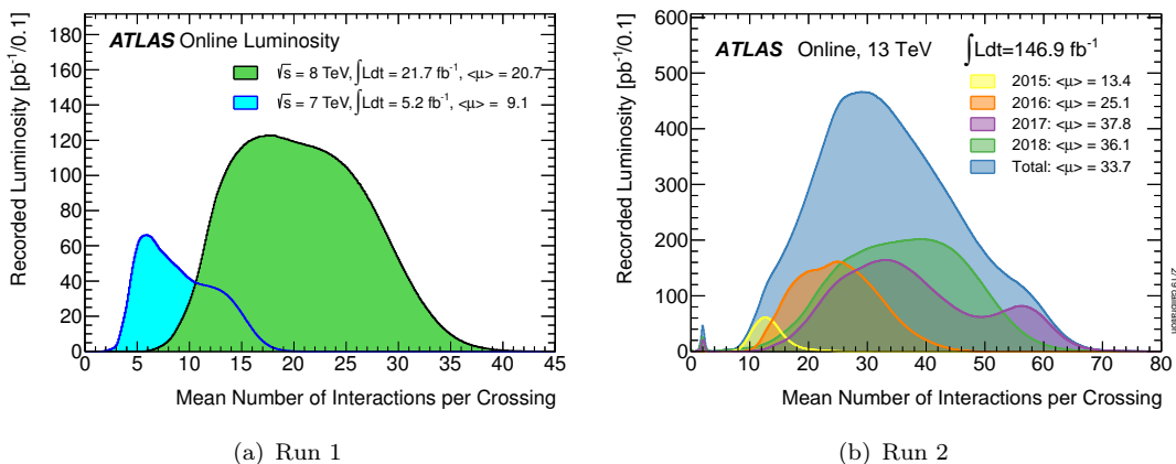
Figure 3.3: Mean number of interactions per bunch crossing for Run 1 (a) and Run 2 (b) of pp collision data at 7, 8 and 13 TeV centre-of-mass energy. Data recorded by the ATLAS detector during stable beams is shown, and the total integrated luminosity and the mean number of interactions per bunch crossing \langle \mu \rangle per year are given in the figures [74, 75].
