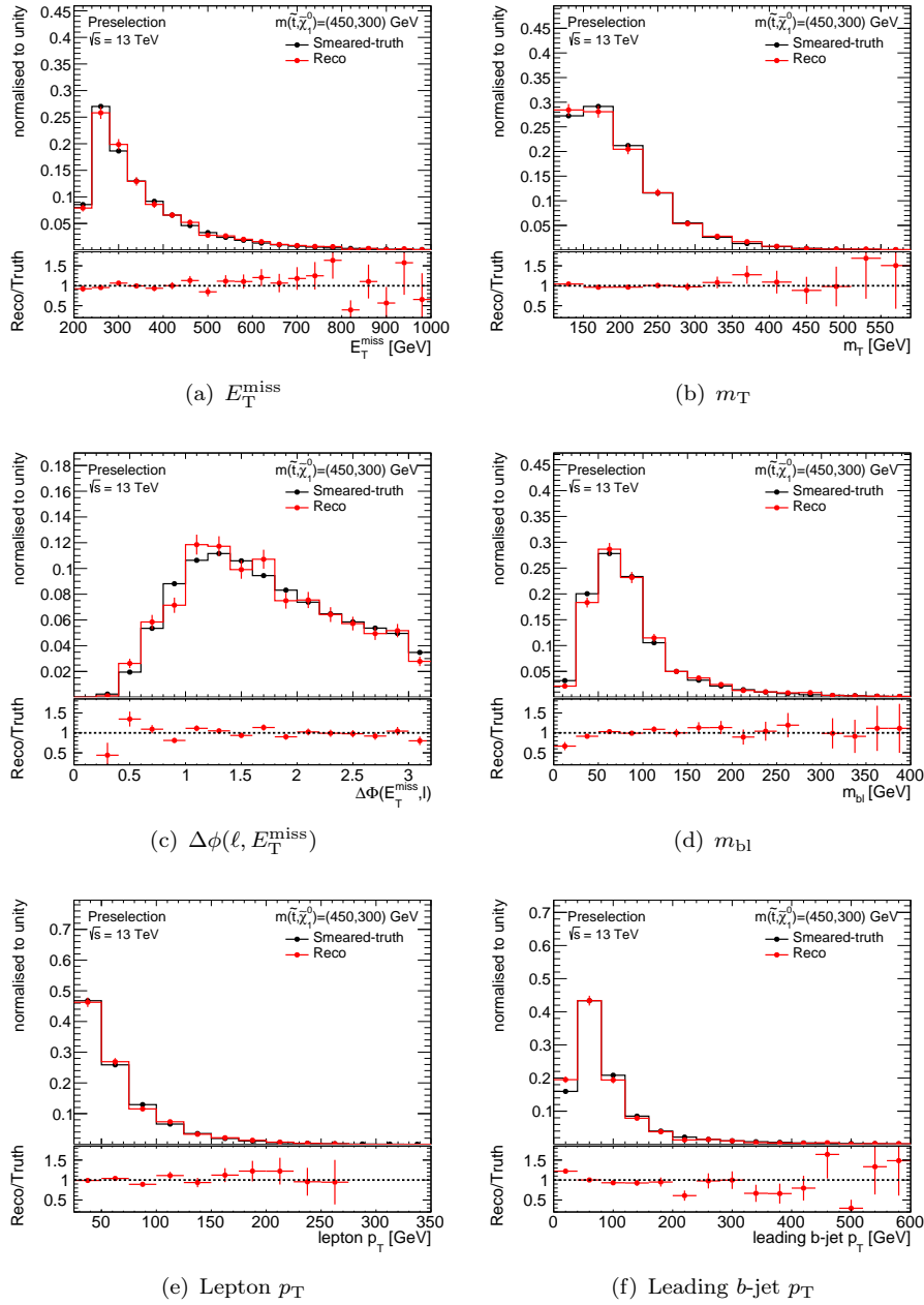
Figure 8.3: Comparison of kinematic distributions between smeared particle-level signal events (“Smeared-truth”, shown as black dots on a black histogram) and fully reconstructed signal events (“Reco” shown as red dots on a red histogram) after preselection. Distributions are normalised to unity in order to investigate the shape of the distributions.
