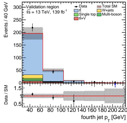
(f) 4 th leading jet p_T
