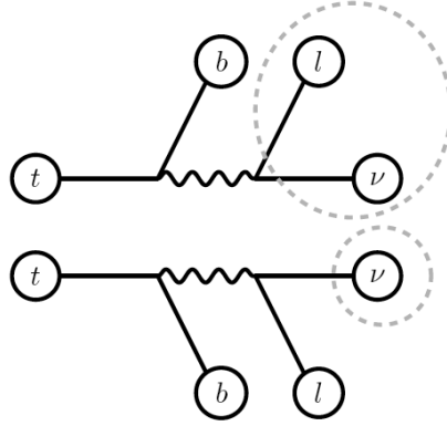
Figure 4.4: Illustration of the construction of m_{T2}^{\tau} , in order to discriminate dileptonic t\bar{t} events with one lost lepton [173].
