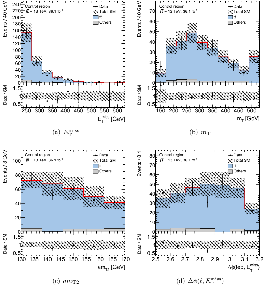
Figure 7.7: Kinematic distributions of key variables for events that pass the control region selection. The t\bar{t} events are scaled by the normalisation factor obtained in the CR. Residual SM background processes are normalised with the respective theoretical cross section. The category ‘Others’ in the legend represents the sum of minor SM backgrounds that contribute less than 5 % of the total SM background. The lower panel shows the ratio of data to the SM prediction. The uncertainty band includes statistical and experimental systematic uncertainties. t\bar{t} modelling uncertainties are only determined for the VR and SR and hence not included in the total uncertainty. The last bins include the overflow.
