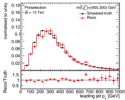
(c) Leading jet p_T
