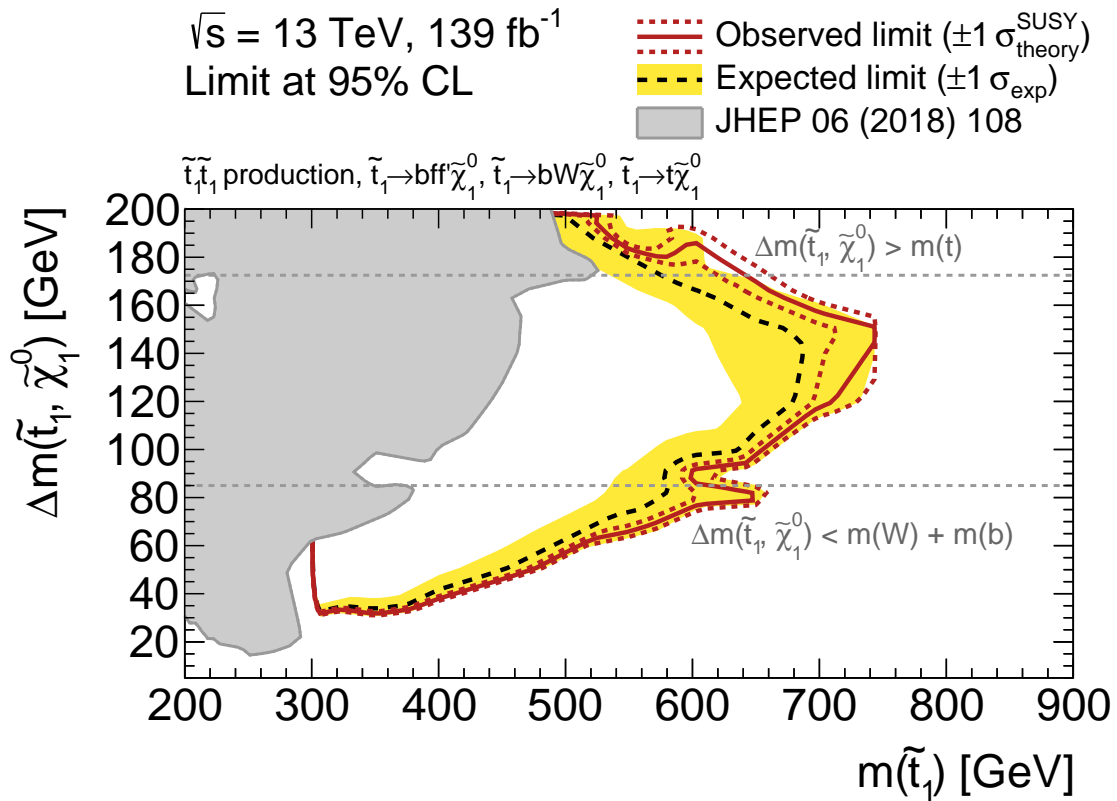
Figure 8.29: Expected (black dashed) and observed (red solid) excluded regions in the plane of \Delta m(\tilde{t}_1, \tilde{\chi}_1^0) versus m(\tilde{t}_1) at 95 % confidence level for direct top squark pair production. Either \tilde{t}_1 \rightarrow t \tilde{\chi}_1^0 , \tilde{t}_1 \rightarrow b W \tilde{\chi}_1^0 , or \tilde{t}_1 \rightarrow b f \tilde{\chi}_1^0 decay modes are assumed with a branching ratio of 100 %. The grey shaded area illustrates excluded regions from a previous publication [58], including also the results obtained from the analysis described in Chapter 7.
