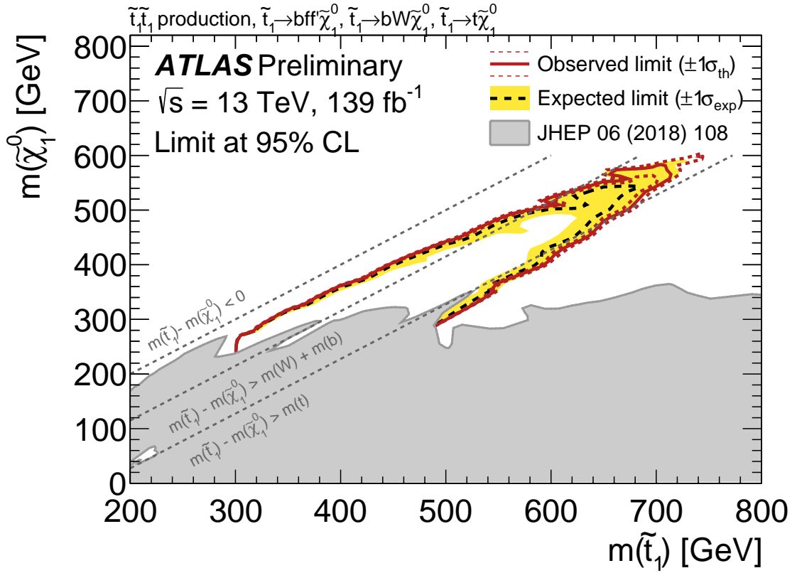
Figure 8.28: Expected (black dashed) and observed (red solid) excluded regions in the plane of m(\tilde{\chi}_1^0) versus m(\tilde{t}_1) at 95 % confidence level for direct top squark pair production. Either \tilde{t}_1 \rightarrow t\tilde{\chi}_1^0 , \tilde{t}_1 \rightarrow bW\tilde{\chi}_1^0 , or \tilde{t}_1 \rightarrow bff'\tilde{\chi}_1^0 decay modes are assumed with a branching ratio of 100 %. The grey shaded area illustrates the excluded region from a previous publication [58], including also the results obtained from the analysis described in Chapter 7.
