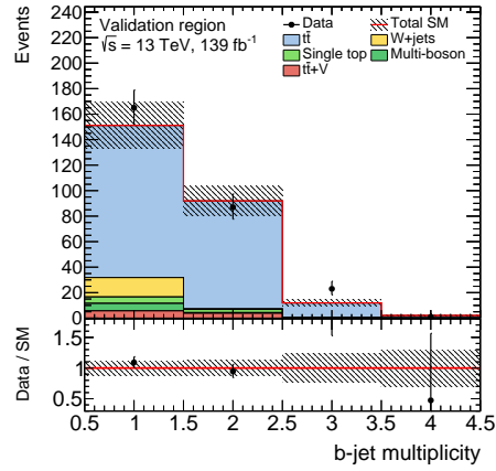
(b) b -jet multiplicity
