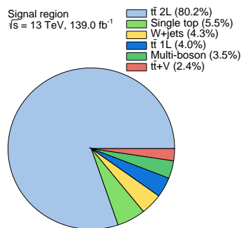
Figure 8.14: Breakdown of the individual SM contributions to the signal region.
