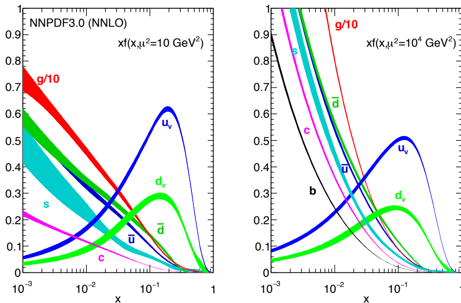
Figure 4.1: Parton distribution functions of the gluon, valence quarks and various sea quarks of the proton obtained in the NNLO NNPDF3.0 global analysis [93]. The left plot corresponds to hadronic scales ( \mu^2 = 10 \text{ GeV}^2 ) and the right plot corresponds to higher scales as present at the LHC ( \mu^2 = 10^4 \text{ GeV}^2 ) [5].
