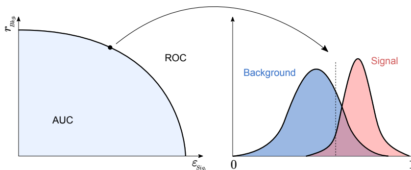
Figure 5.8: Receiver operating characteristic. The ROC can be derived from the distribution of the output activation of signal and background events.
