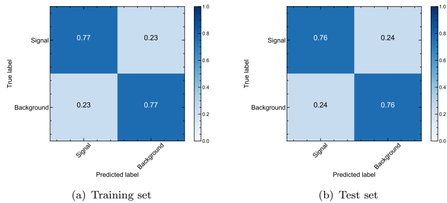
Figure 8.9: Confusion matrices of training set and test set. The values in the diagonal and off-diagonal terms represent the fraction of correctly and misidentified events of both classes.
