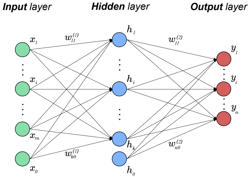
Figure 5.1: Basic structure of a multilayer perceptron, which consists of an input layer, an individual amount of hidden layers and an output layer. The various layers in turn are build up from single neurons, representing for example input variables of the data set or predicted outputs.
