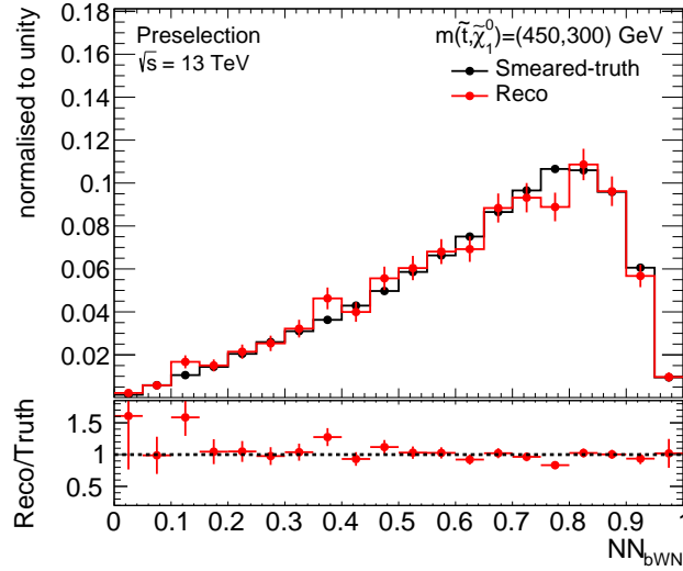
Figure 8.11: Comparison of the distribution of the ML output score between particle-level and reconstructed events of the benchmark signal model. Both distributions agree well within uncertainty. In order to investigate differences of the shapes of the distributions, the distributions are normalised to unity.
