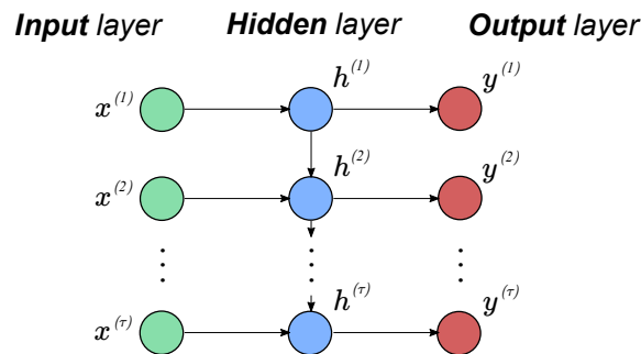
Figure 5.4: Unfolding of a single neuron of a hidden layer in a RNN. The unfolded neuron does not necessarily need a connection to the output neuron at each sequence. Instead, only a single output neuron at the end of the sequence is also viable.
