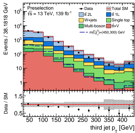
(e) 3 rd leading jet p_T
