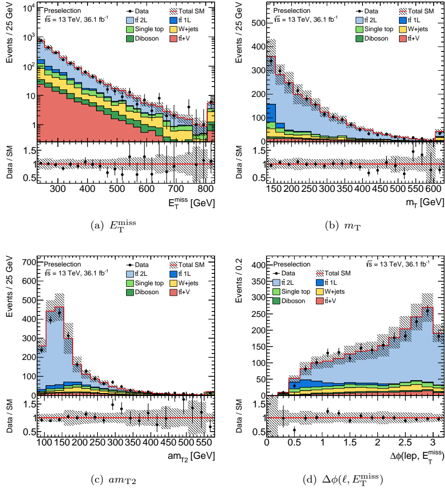
Figure 7.2: Kinematic distributions of key observables after the preselection is applied. The t\bar{t} background prediction is scaled by the normalisation factor obtained from a likelihood fit of the CR, while all other SM background processes are normalised with the respective theoretical cross sections. The hatched band around the total SM prediction and the hatched band in the data/SM ratio include statistical and systematic uncertainties, except the t\bar{t} modelling uncertainties, which are determined only for the VR and SR, respectively. Overflows are included in the last bin.
