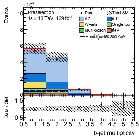
(b) b -jet multiplicity
