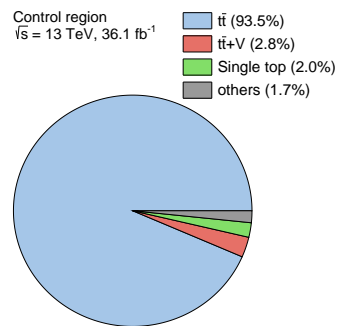
Figure 7.6: Relative contributions of the individual SM backgrounds in the control region.
