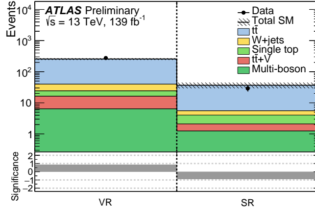
Figure 8.25: Comparison of observed events with the SM prediction in the VR and SR. The shaded area around the total SM background prediction includes all uncertainties. The bottom panel shows the significance of the observed data events given the number of predicted SM background events.
