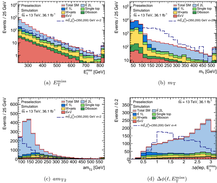
Figure 7.3: Kinematic distributions of the most important variables of the analysis after the preselection. Only simulated events are shown. For the distribution of m_T , the cut on the shown quantity is omitted in the event preselection in order to stress the discriminating power of this observable. Only statistical uncertainties are shown in the distributions. Overflows are included in the last bin. The distribution for signal events is scaled by multiples of its nominal cross section, to illustrate the distinct kinematics compared to the SM background.
