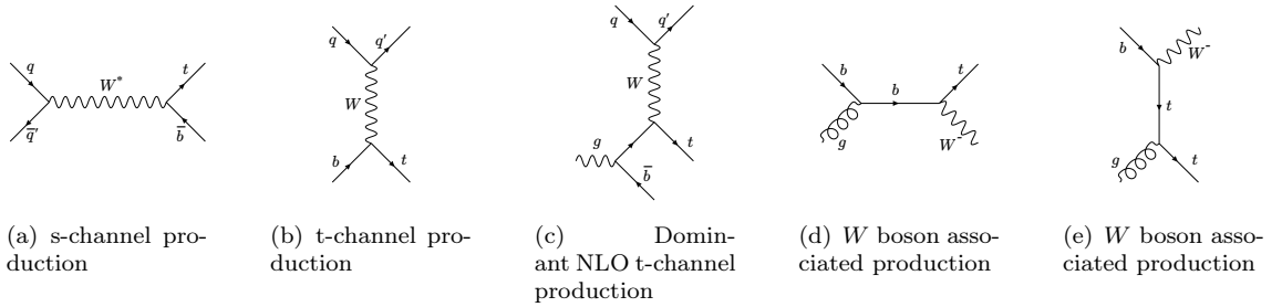
Figure 4.3: Feynman diagrams for the production of single top quarks.
