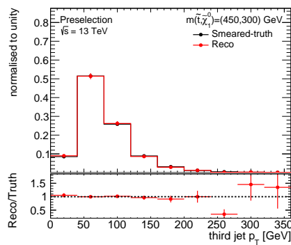
(e) 3 rd leading jet p_T
