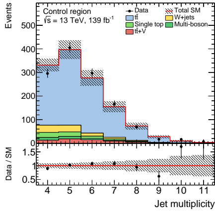
(a) Jet multiplicity
