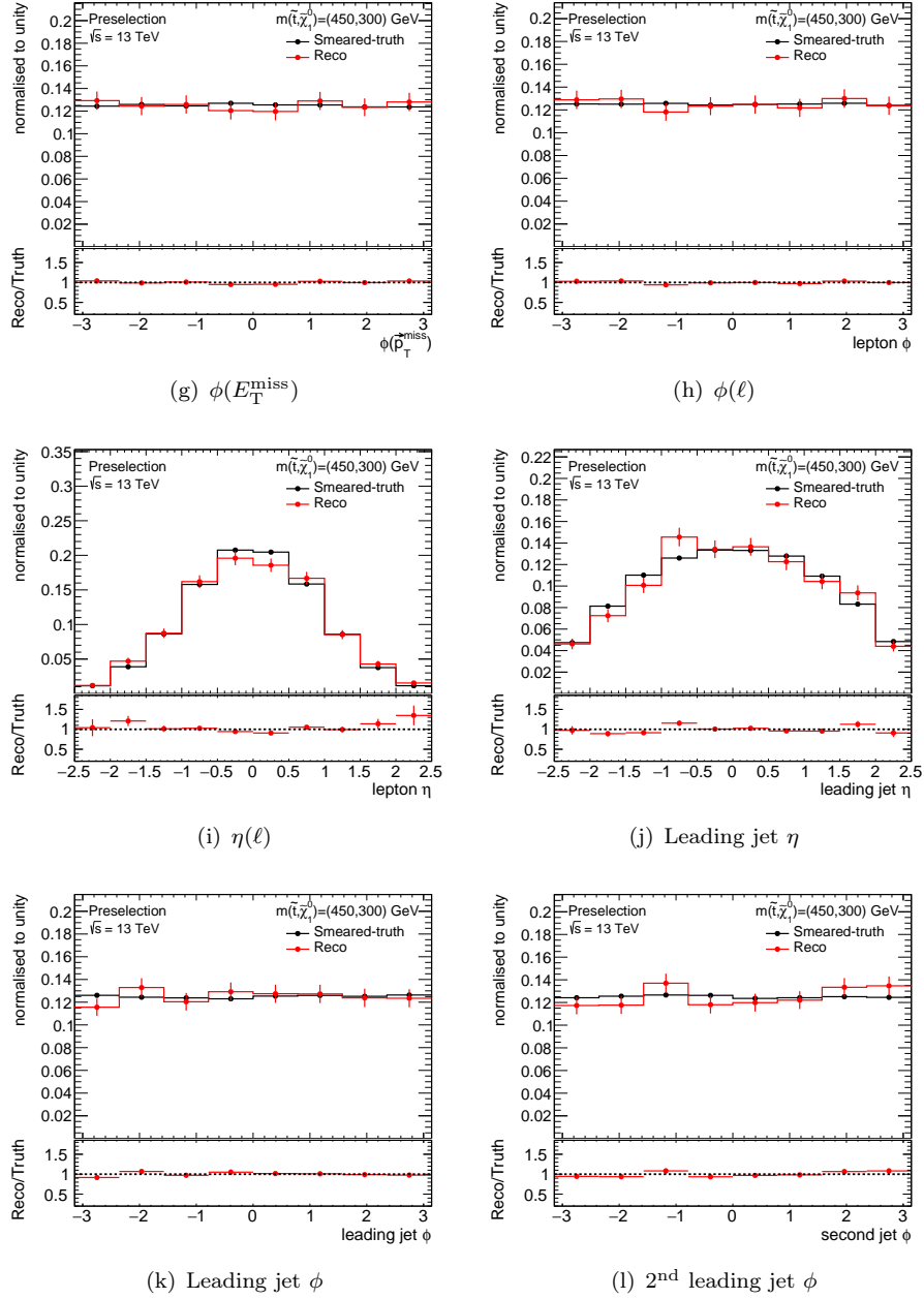
Figure A.2: Comparison of kinematic distributions between smeared particle-level signal events (“Smeared-truth”, shown as black dots on a black histogram) and fully reconstructed signal events (“Reco” shown as red dots on a red histogram) after preselection. Distributions are normalised to unity in order to investigate the shape of the distributions.
