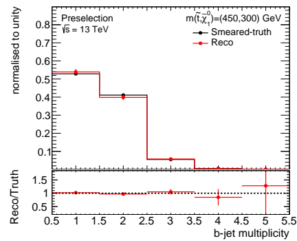
(b) b -jet multiplicity
