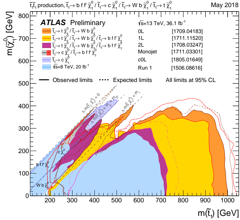
Figure 2.7: Summary of the individual ATLAS searches for top squark pair production based on 36.1 \text{ fb}^{-1} of pp collision data at a centre-of-mass energy 13 TeV [64]. Exclusion limits at 95 % confidence level are shown in the m(\tilde{t}_1) versus m(\tilde{\chi}_1^0) mass plane. The dashed and solid lines show the expected and observed limits, respectively. For the derived limits, statistical as well as systematic uncertainties except for the theoretical signal cross section uncertainty are included. Different decay modes are considered separately with a branching ratio of 100 %, respectively: \tilde{t}_1 \rightarrow t\tilde{\chi}_1^0 , \tilde{t}_1 \rightarrow bW\tilde{\chi}_1^0 , \tilde{t}_1 \rightarrow bff\tilde{\chi}_1^0 and \tilde{t}_1 \rightarrow c\tilde{\chi}_1^0 . The latter two decay modes are superimposed.
