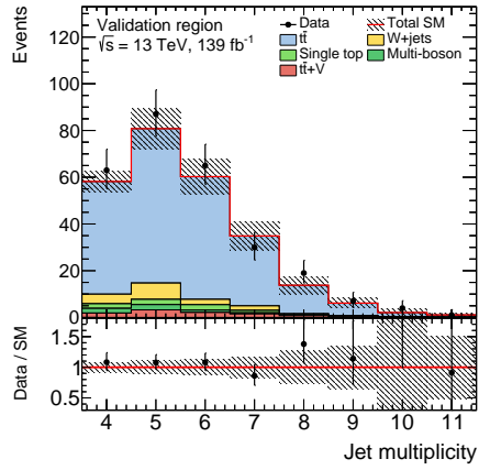
(a) Jet multiplicity
