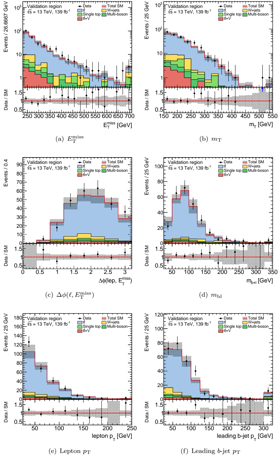
Figure 8.24: Kinematic distributions of selected observables in the validation region. The t\bar{t} background processes are scaled by the normalisation factor obtained from a likelihood fit of the CR, while all other SM background processes are normalised with the respective theoretical cross section. The shaded band around the total SM prediction as well as the shaded band in the data/SM ratio include statistical and systematic uncertainties. Overflows are included in the last bin.
