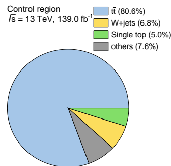
Figure 8.19: Relative contributions of the individual SM backgrounds in the control region.
