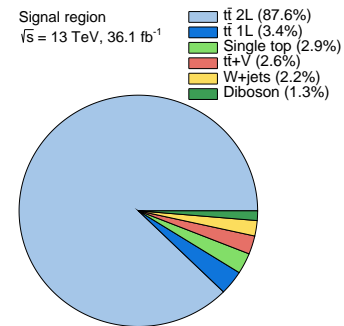
Figure 7.4: Relative contributions of the individual SM backgrounds in the signal region.
