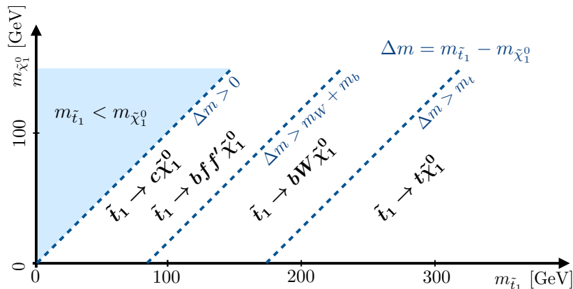
Figure 2.6: Illustration of the preferred top squark decay modes, assuming that the top squarks decay into a bino-like neutralino. The phase space of interest is spanned by the masses of the top squark ( m(\tilde{t}_1) ) and the lightest neutralino ( m(\tilde{\chi}_1^0) ) [55].
