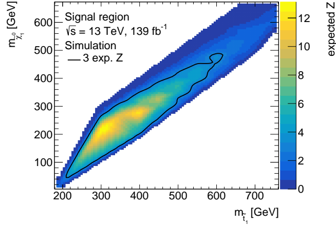
Figure 8.15: Expected significance across the signal phase space spanned by m(\tilde{t}_1) versus m(\tilde{\chi}_1^0) . The considered phase space spans over signal points characterised by 20 \text{ GeV} < \Delta m < 200 \text{ GeV} . The black contour line illustrates the threshold for Z > 3 .
