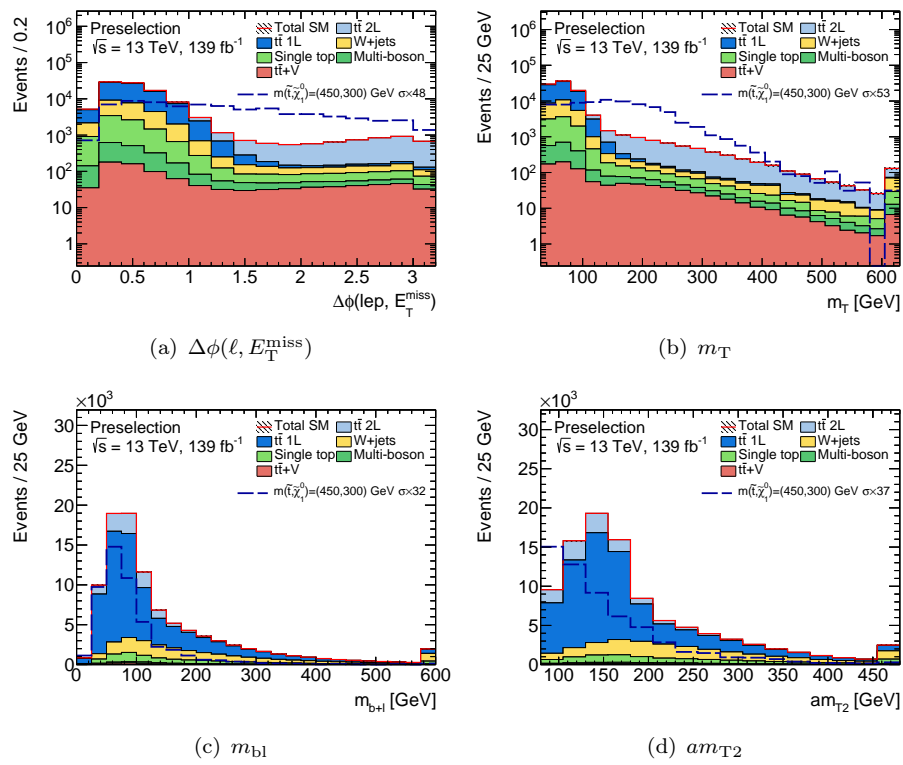
Figure 4.6: Distributions of the discriminating variables after the preselection as described in Table 8.1 except for the threshold on m_T which is loosened to m_T \geq 30 \text{ GeV} . The object definitions from the bWN-fullSet analysis are used. The cross section of the SUSY signal is magnified in order to stress the discriminating power of the variable.
