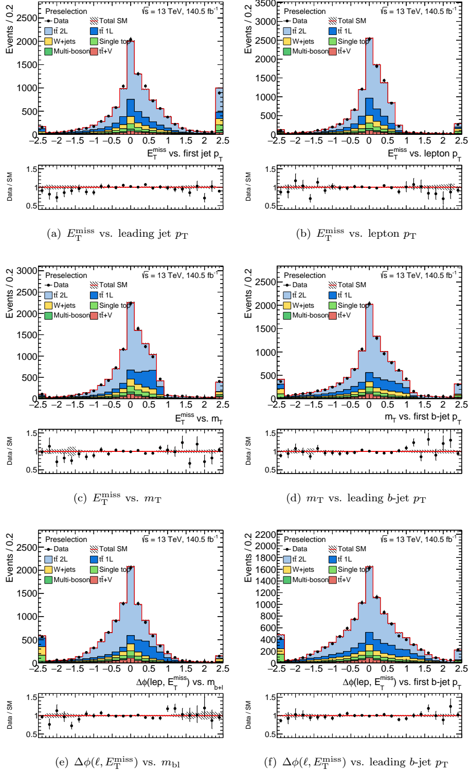
Figure 8.5: Distributions of the linear correlation between two kinematic observables, respectively. Agreement between data and simulated background events is observed. Only statistical uncertainties are shown. Underflows and overflows are included in the first and last bins.
