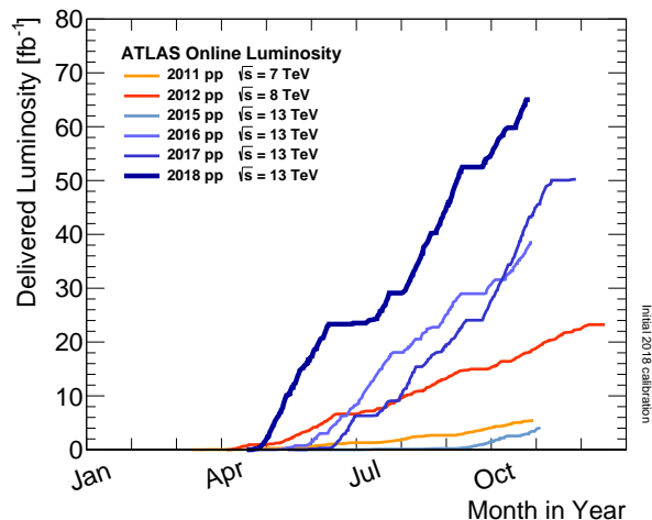
Figure 3.2: Integrated luminosity of stable beams for pp collisions delivered to ATLAS over the period of twelve months [74].
