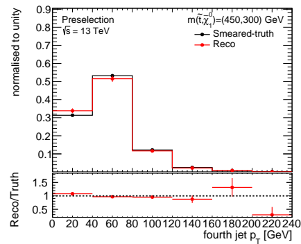
(f) 4 th leading jet p_T
