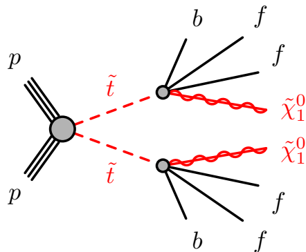
Figure 2.5: Simplified model topology of direct top squark pair production in a highly compressed phase space. The mass difference between the supersymmetric particles is so small ( \Delta m < m(W) + m(b) ), that the top quark as well as the W boson can only be produced off-shell and thus the top squarks decay via a 4-body decay mode. By courtesy of the ATLAS supersymmetry physics analysis group.
