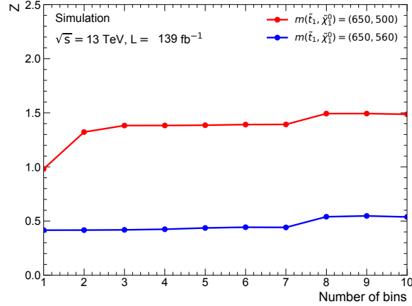
Figure 8.17: Expected significance Z for rejecting the background+signal hypothesis for two different signal points as a function of bins included to the maximum likelihood fit. Z significantly increases if multiple bins are added to the fit procedure. Proper systematic uncertainties accounting for t\bar{t} radiation, fragmentation and hard scattering are applied respectively, as well as systematic uncertainties for flavor tagging, lepton identification, isolation and reconstruction, and pileup are included. E_T^{\text{miss}} uncertainties as well as uncertainties on jet energy scales and resolutions are also applied. Signal acceptance uncertainties and uncertainties on the cross section of the minor SM backgrounds are included as well.
