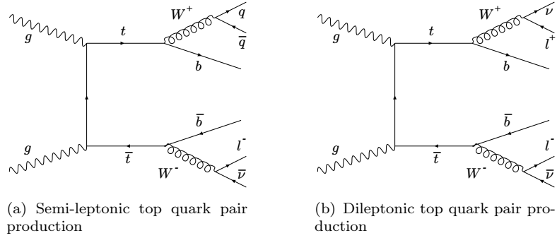
Figure 4.2: Feynman diagrams of top quark pair production and decay.
