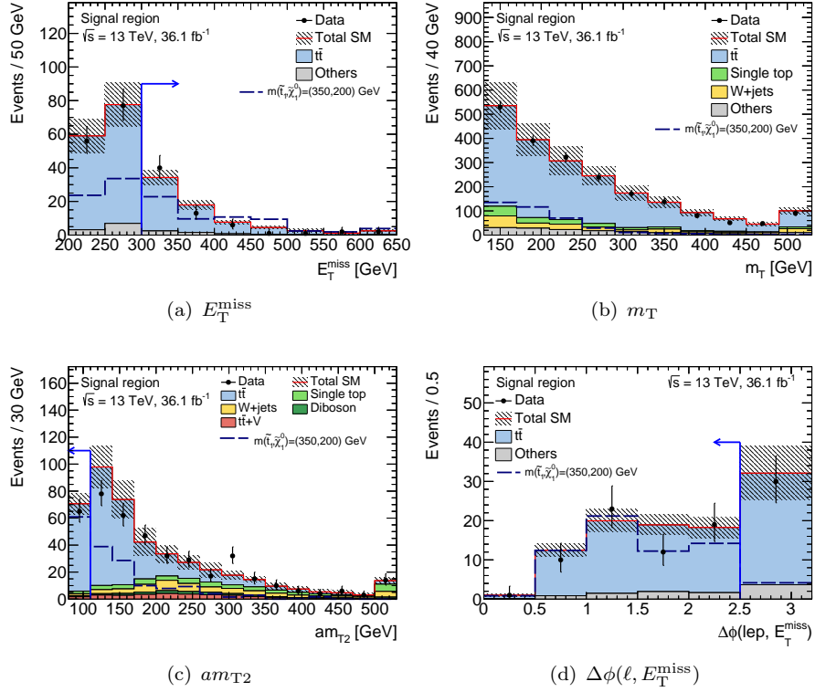
Figure 7.11: Kinematic distribution of relevant variables in the signal region. The requirement on the plotted quantity is omitted, but indicated by the vertical lines, except for the m_T distribution. The predicted t\bar{t} background process is scaled with the normalisation factor obtained from the control region. Furthermore, the benchmark signal model is shown. The label ‘Others’ in the legend represents minor SM backgrounds that contribute less than 5% of the total background. All uncertainties are included and represented by the shaded area around the total SM expectation. The last bin contains overflows.
