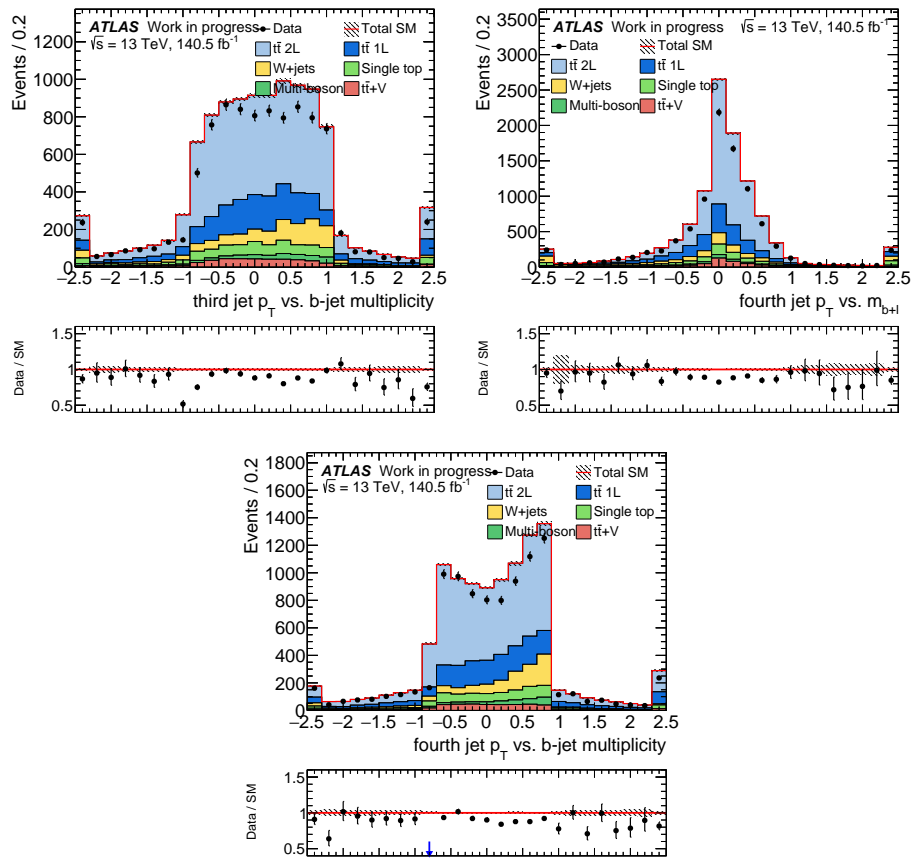
Figure A.2: Distributions of the linear correlation between two kinematic observables, respectively. Agreement between data and simulated background events is observed. Only statistical uncertainties are shown. Underflows and overflows are included in the first and last bins.
