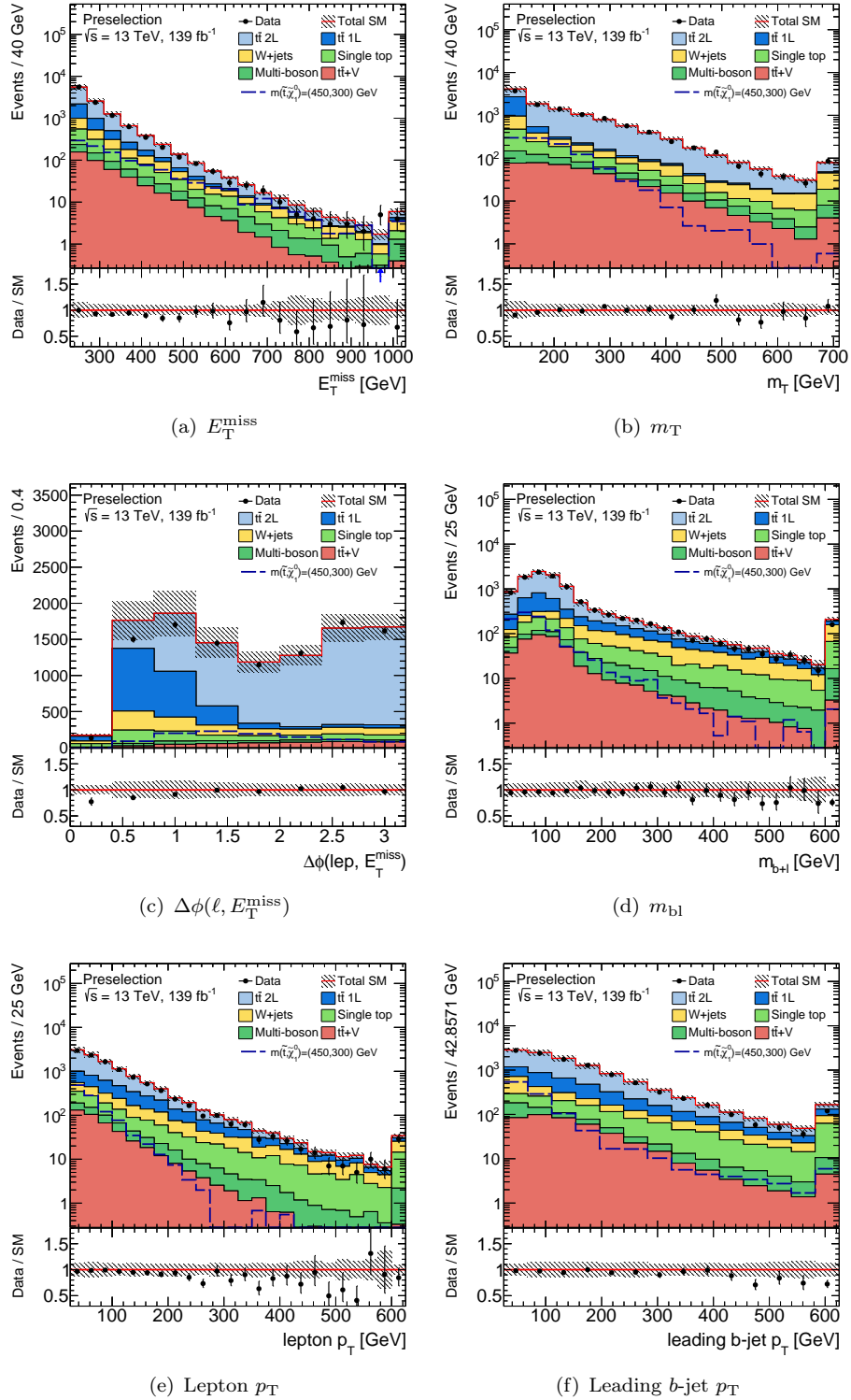
Figure 8.2: Kinematic distributions of key observables after the preselection is applied. The t\bar{t} background prediction is scaled by the normalisation factor obtained from a likelihood fit of the CR, while residual SM background processes are normalised with the respective theoretical cross section. The hatched area around the total SM prediction and the hatched band in the ratio include statistical and systematic uncertainties, except for the t\bar{t} modelling uncertainties, which are defined only for the signal and validation region. Additionally, the expected distribution of the SUSY benchmark signal model is overlaid (blue dashed line). Overflows are included in the last bin.
