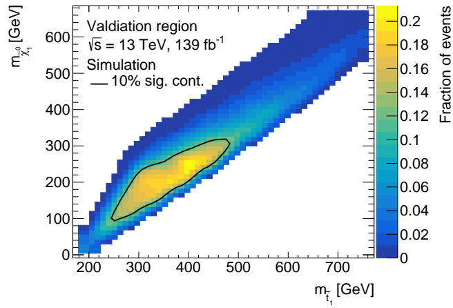
Figure 8.23: Signal contamination in the validation region illustrated in the phase space spanned by m(\tilde{t}_1) versus m(\tilde{\chi}_1^0) . The black contour line illustrates the threshold for a signal fraction of 10%. Signal points where the contamination is above 10% are already excluded by previous analyses.
