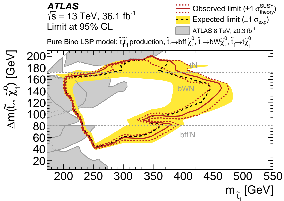
Figure 7.14: Expected (black dashed) and observed (red solid) 95% excluded regions in the plane of \Delta m(\tilde{t}_1, \tilde{\chi}_1^0) versus m(\tilde{t}_1) for direct top squark pair production assuming either \tilde{t}_1 \rightarrow t \tilde{\chi}_1^0 , \tilde{t}_1 \rightarrow bW \tilde{\chi}_1^0 , or \tilde{t}_1 \rightarrow bff' \tilde{\chi}_1^0 decay with a branching ratio of 100%. The excluded regions from previous publications [55, 173] are also illustrated with the grey shaded area.
