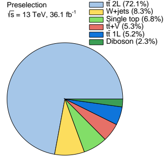
Figure 7.1: Relative contributions of the individual SM backgrounds after the preselection.
