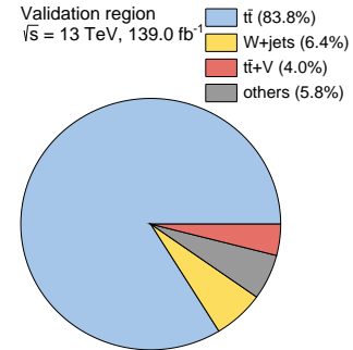
Figure 8.22: Relative contributions of the individual SM backgrounds in the validation region.
