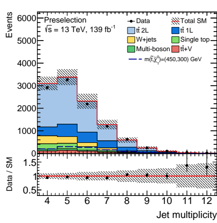
(a) Jet multiplicity
