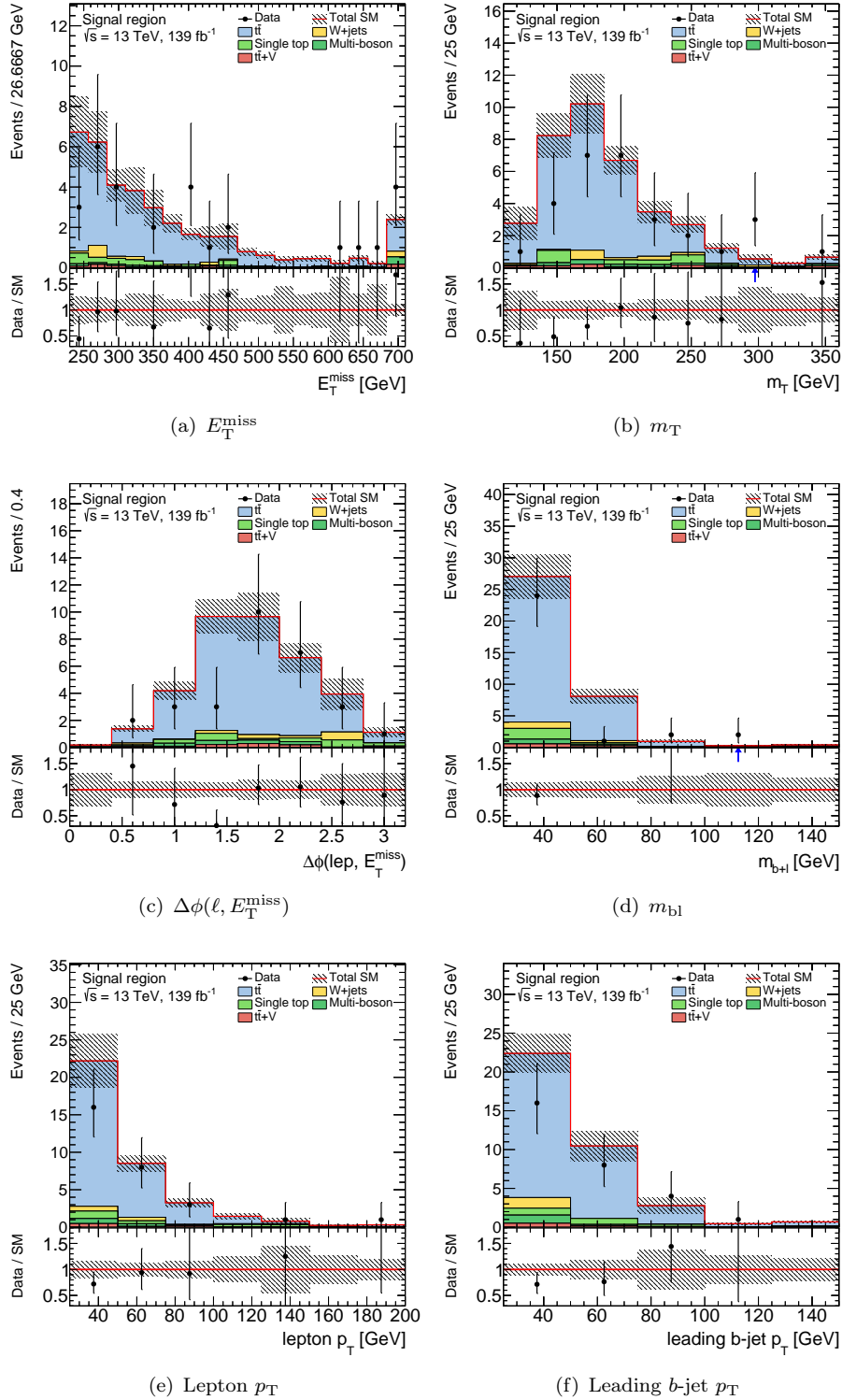
Figure 8.26: Kinematic distributions of selected observables in the signal region. The t\bar{t} background processes are scaled by the normalisation factor obtained from a likelihood fit of the CR, while all other SM background processes are normalised with the respective theoretical cross section. The shaded band around the total SM prediction as well as the shaded band in the data/SM ratio include statistical and systematic uncertainties. Overflows are included in the last bin.
