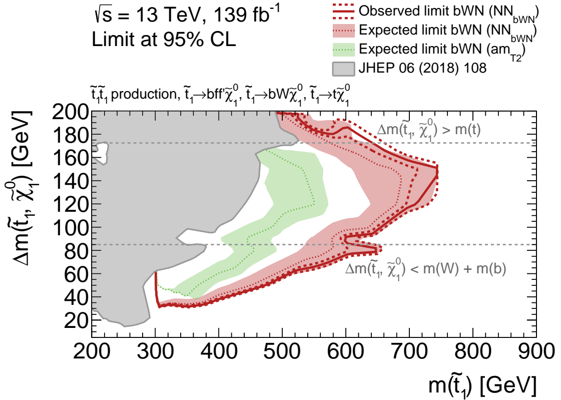
Figure 9.2: Comparison of the expected (green dashed) excluded region obtained from a shape-fit in \text{am}_{\text{T2}} with the expected (red dashed) and observed (red solid) excluded regions derived from a shape-fit in \text{NN}_{\text{bWN}} in the plane of \Delta m(\tilde{t}_1, \tilde{\chi}_1^0) versus m(\tilde{t}_1) for direct top squark pair production. The limits correspond to 95 % confidence level. Either \tilde{t}_1 \rightarrow t\tilde{\chi}_1^0 , \tilde{t}_1 \rightarrow bW\tilde{\chi}_1^0 , or \tilde{t}_1 \rightarrow bff'\tilde{\chi}_1^0 decay modes with a branching ratio of 100 % are assumed. The excluded region from the previous publication [55] is illustrated as the grey shaded region.
