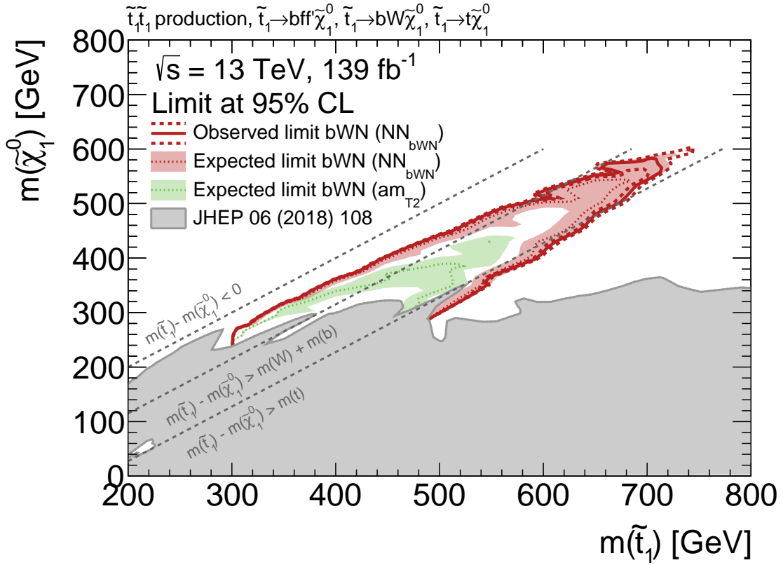
Figure 9.1: Comparison of the expected (green dashed) excluded region obtained from a shape-fit in \text{am}_{\text{T}2} with the expected (red dashed) and observed (red solid) excluded regions derived from a shape-fit in \text{NN}_{\text{bWN}} in the plane of m(\tilde{t}_1) versus m(\tilde{\chi}_1^0) for direct top squark pair production. The limits correspond to 95 % confidence level. Either \tilde{t}_1 \rightarrow t \tilde{\chi}_1^0 , \tilde{t}_1 \rightarrow b W \tilde{\chi}_1^0 , or \tilde{t}_1 \rightarrow b f f' \tilde{\chi}_1^0 decay modes with a branching ratio of 100 % are assumed. The excluded region from the previous publication [55] is illustrated as the grey shaded region.
