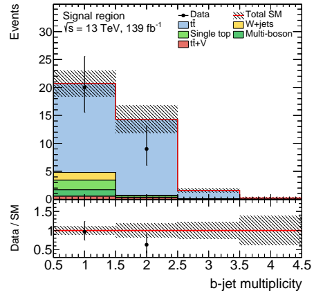
(b) b -jet multiplicity
