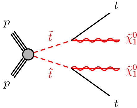
Figure 2.3: Simplified model topology of direct top squark pair production. The top squark directly decays to a top quark and the neutralino LSP. \tilde{\chi}_1^0 is predominantly bino-like. By courtesy of the ATLAS supersymmetry physics analysis group.
