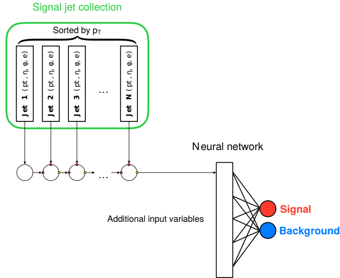
Figure 8.4: Conceptual layout of the machine learning architecture used to discriminate signal from SM background. In order to exploit the information of the whole jet collection, jet 4-vectors are processed in a recurrent neural network. The output vector of the jet-RNN is then passed as an input to the NN together with further discriminating variables.
