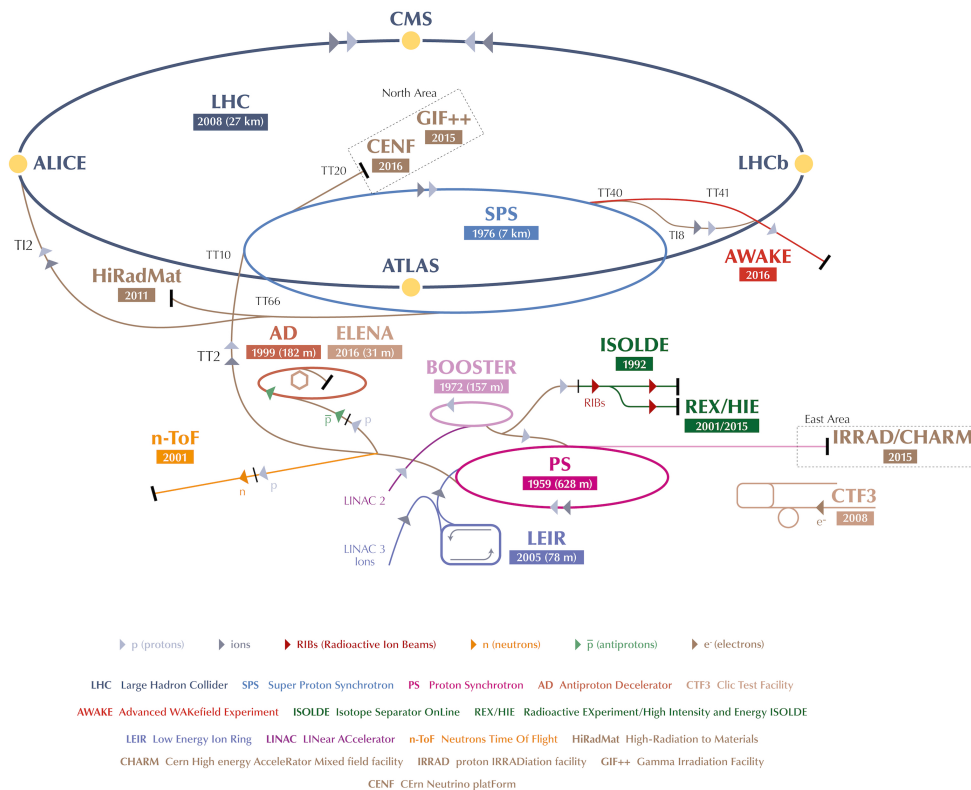
Figure 3.1: CERN accelerator complex [66]. At first, protons are accelerated by the LINAC2 to energies up to 50 MeV, afterwards further acceleration up to 1.4 GeV is achieved by the BOOSTER followed by the PS (26 GeV). In the SPS they got accelerated up to 450 GeV and finally injected in the LHC where they are able to achieve a maximum energy of 7 TeV.
