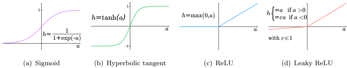
Figure 5.2: Examples of activation functions h used to transform activations a in a dedicated layer.
