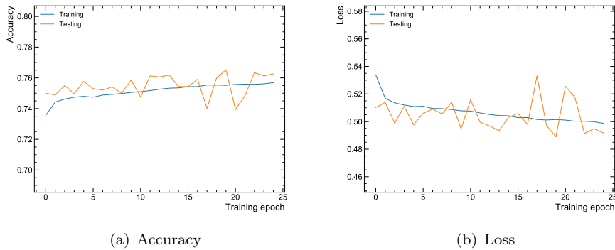
Figure 8.6: Distribution of the accuracy and loss of the NN as a function of the number of training epochs.
