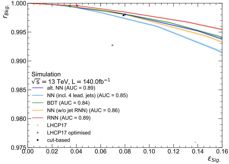
Figure 8.12: Illustration of the ROC curves and working points, associated with a signal region, of the primary ML classifier and various alternative methods.
