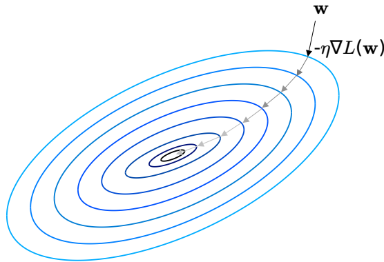
Figure 5.5: Stochastic gradient descent. The ellipses represent contours in the weight space. By iteratively updating the weights with respect to the actual gradient of the loss function, the trajectory is moving towards the minimum.
