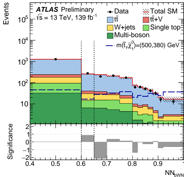
Figure 8.27: Distribution of NN_{bWN} . The variable bin widths correspond to the definitions of the control, validation and signal regions. The shaded area around the total SM prediction includes all uncertainties. The expected distribution from a representative signal benchmark model is overlaid. The bottom panel shows the significance of the observed data events given the number of predicted SM background events.
