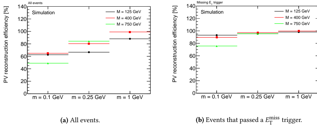
Figure 6.2: PV reconstruction efficiency for various signal models before and after the trigger selection.
