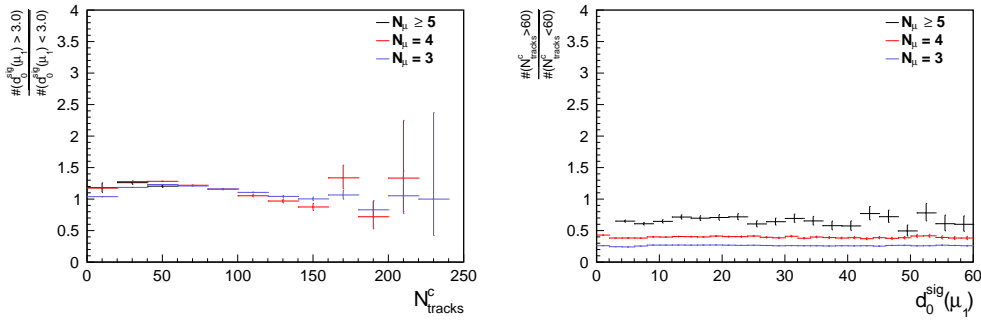
Figure 4.17: Ratio of the number of events with d_0^{\text{sig}}(\mu_1) > 3.0 over the number of events with d_0^{\text{sig}}(\mu_1) < 3.0 (left) and ratio of the number of events with N_{\text{tracks}}^c > 60 over the number of events with N_{\text{tracks}}^c < 60 (right) for data with preselections requiring N_\mu = 3, 4 or N_\mu \geq 5
