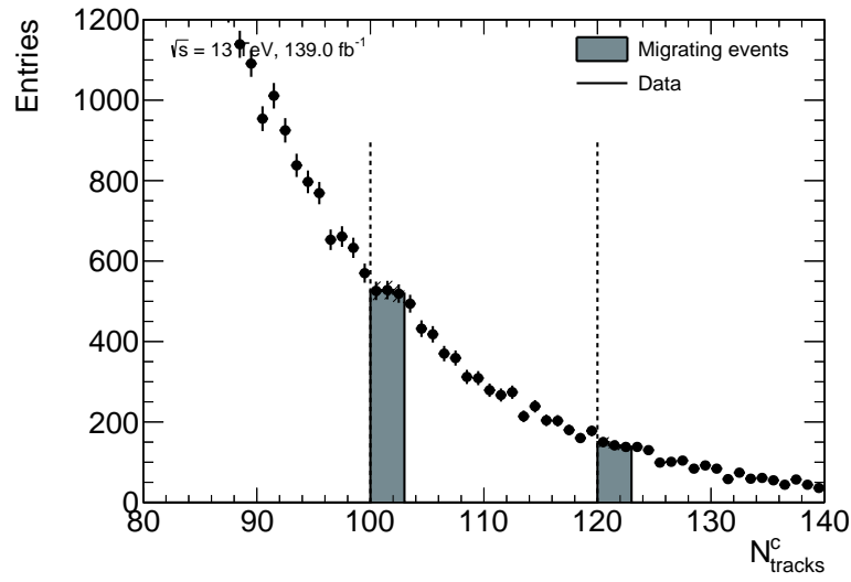
Figure 5.2: Data distribution of N_{\text{tracks}}^c for the preselection requiring N_\mu = 4 and for d_0^{\text{sig}}(\mu_1) < 3 . The dotted lines indicate the position of the VR bin D_{V3}^{4\mu} and the grey areas indicate events that are within N_{\text{tracks}}^c = 3 below the lower or upper limits of the bin.
