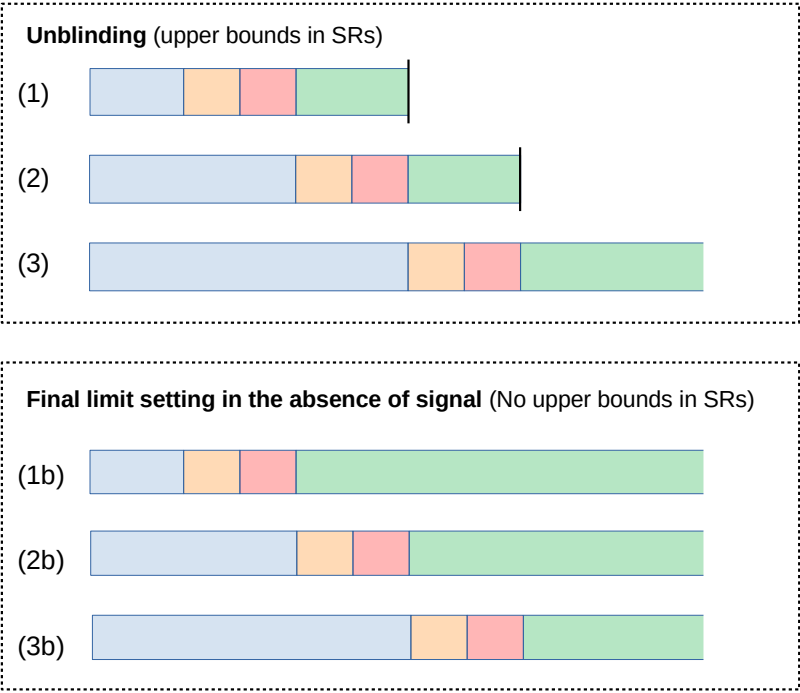
Figure 4.20: Schematic description of the incremental unblinding strategy.
