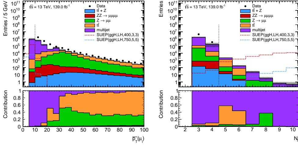
Figure 4.15: Distribution (top) and relative background contributions (bottom) of \bar{p}_T(\mu_i) (left) and N_\mu (right).
