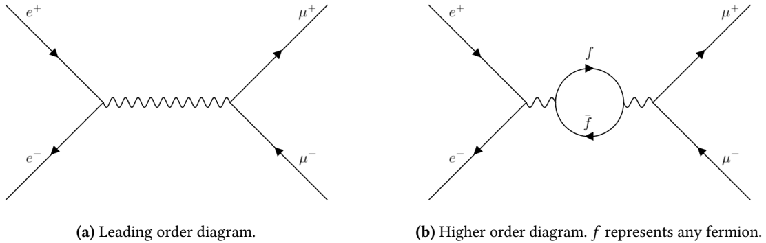
Figure 1.1: Feynman diagrams of e^+e^- \rightarrow \mu^+\mu^- .
