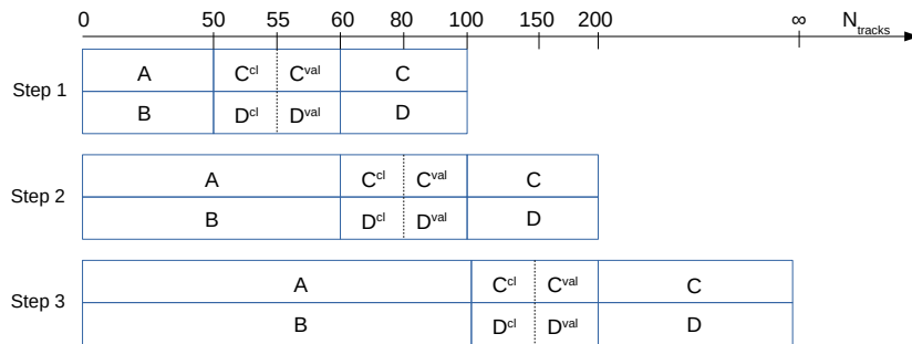
Figure A.1: ABCD regions for each unblinding step
