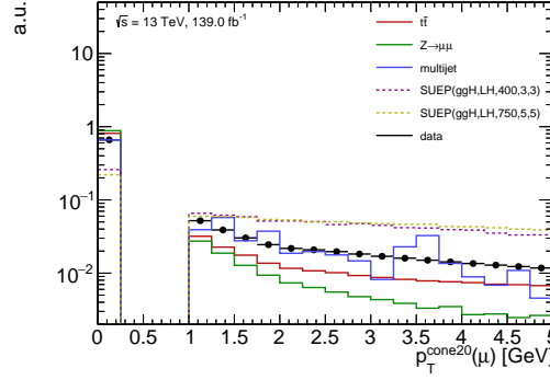
Figure 4.5: p_T^{\text{cone20}} distributions of Low- p_T muons with |\eta| < 2.5 and p_T > 3 GeV using events that passed the HLT_3mu6 trigger for data and Z \rightarrow \mu\mu , t\bar{t} , multijet and two signal samples.
