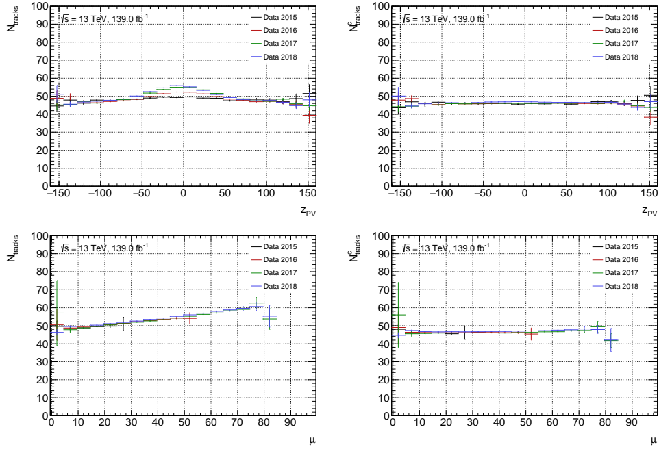
Figure 4.12: N_{\text{tracks}} (left) and N_{\text{tracks}}^c (right) as a function of z_{\text{PV}} (top) and \mu (bottom) for different years of data-taking.
