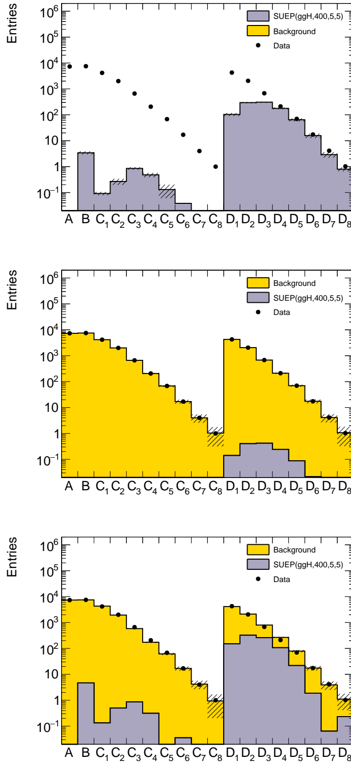
Figure 5.3: Background, SUEP(ggH, LH, 400, 5, 5) signal, and data yields before the fit (top), after the fit with free floating signal strength (middle), and after the fit with fixed signal strength (bottom). Data in the SRs is replaced by the expected background under the H_b hypothesis.
